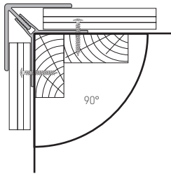
FS-222 Universal corner, 2-piece
